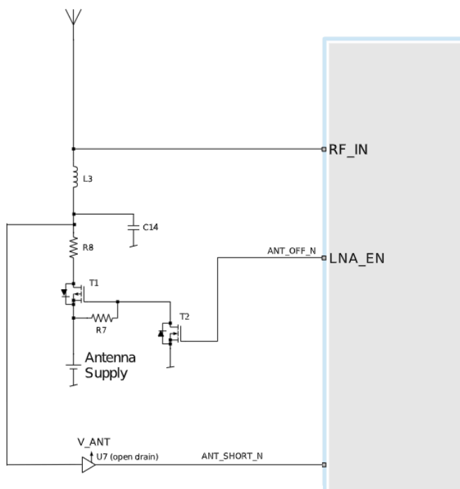
Figure 11: MAX-M10S two-pin antenna supervisor
