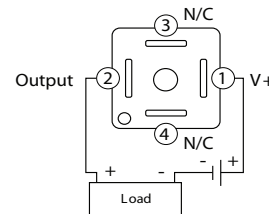
4-20mA Output
