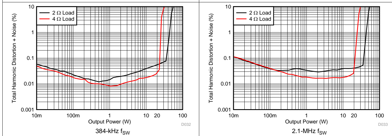
Figure 27. PBTL THD+N vs Power
