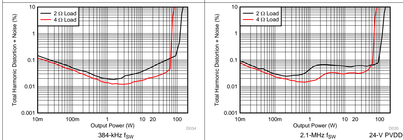
Figure 29. PBTL THD+N vs Power
