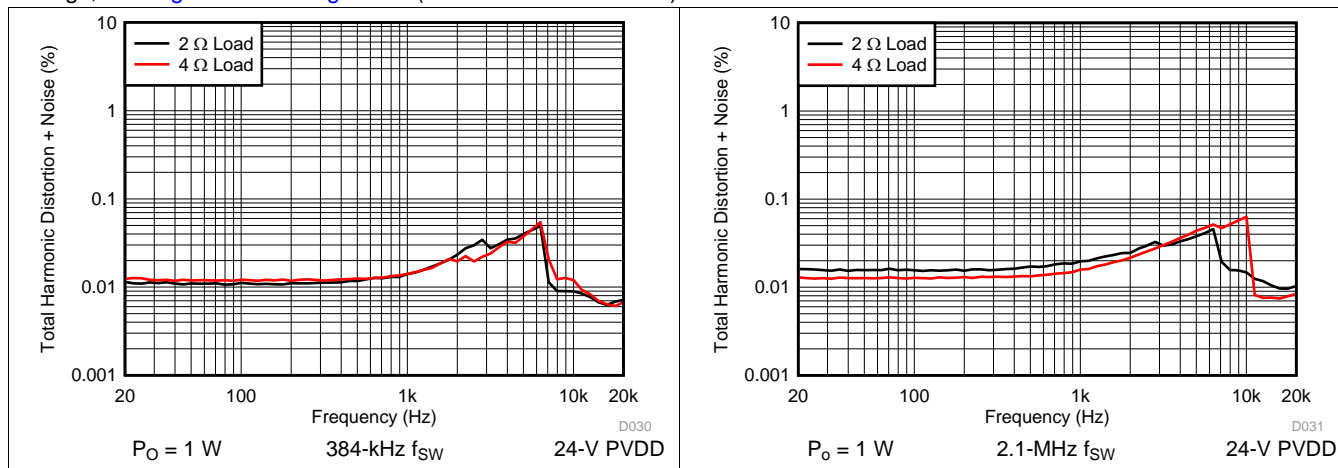
Figure 25. PBTL THD+N vs Frequency
