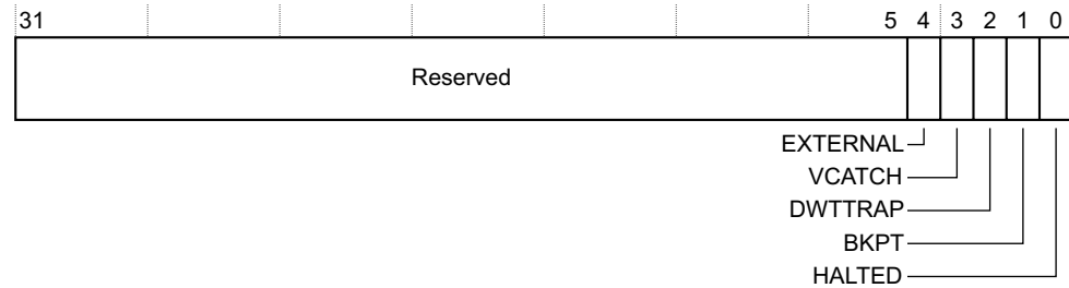
Figure C1-2 DFSCR bit assignments
