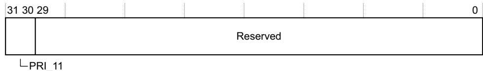
Figure B3-7 SHPR2 Register bit assignments
