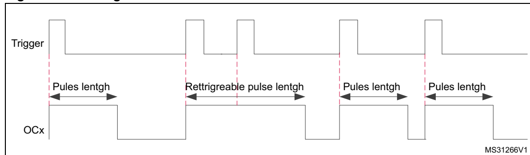
Figure 3. Retriggerable OPM mode
