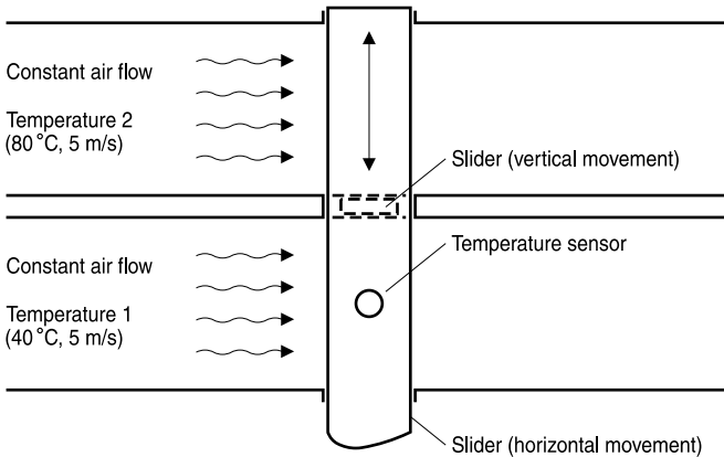
Figure 9 Measurement of thermal time constant in air
