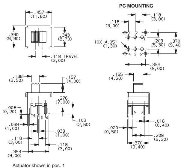
OS202013MT5QN1 DPDT
