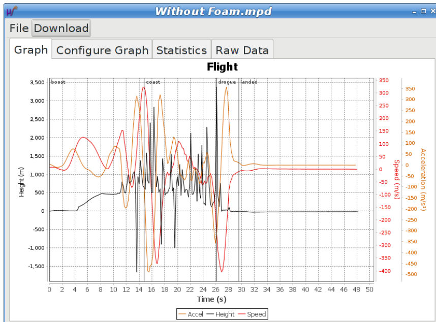
Figure 13. MicroPeak in Sunlight
