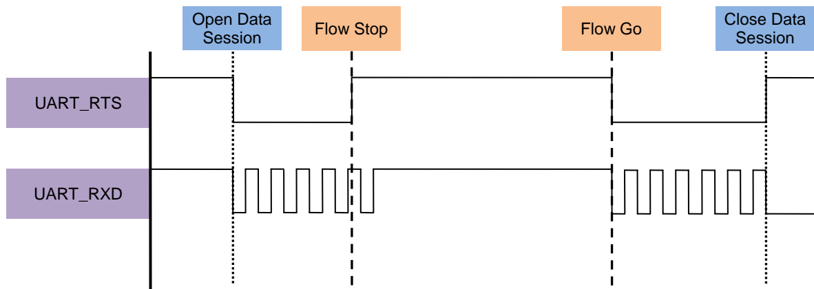
Fig 2.5.2 BLEDK3 indicate Host MCU UART flow control timing diagram
