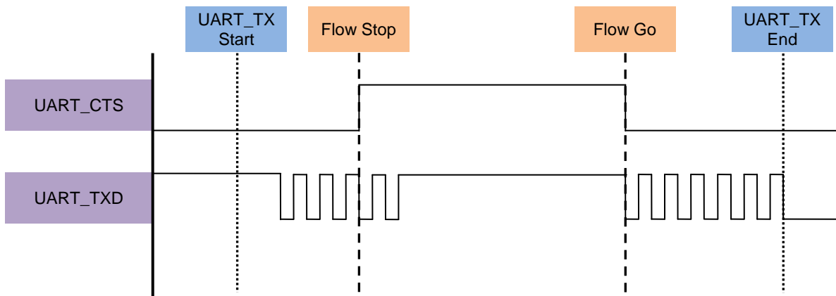
Fig 2.5.1 Host MCU indicate BLEDK3 UART flow control timing diagram
