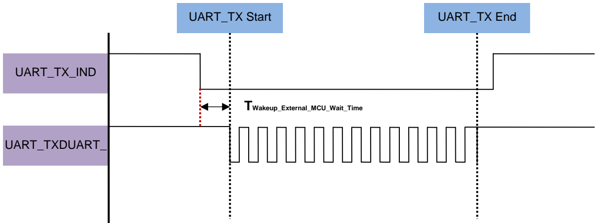
Fig 2.4.2 BLEDK3 indicate Host MCU UART data timing diagram
