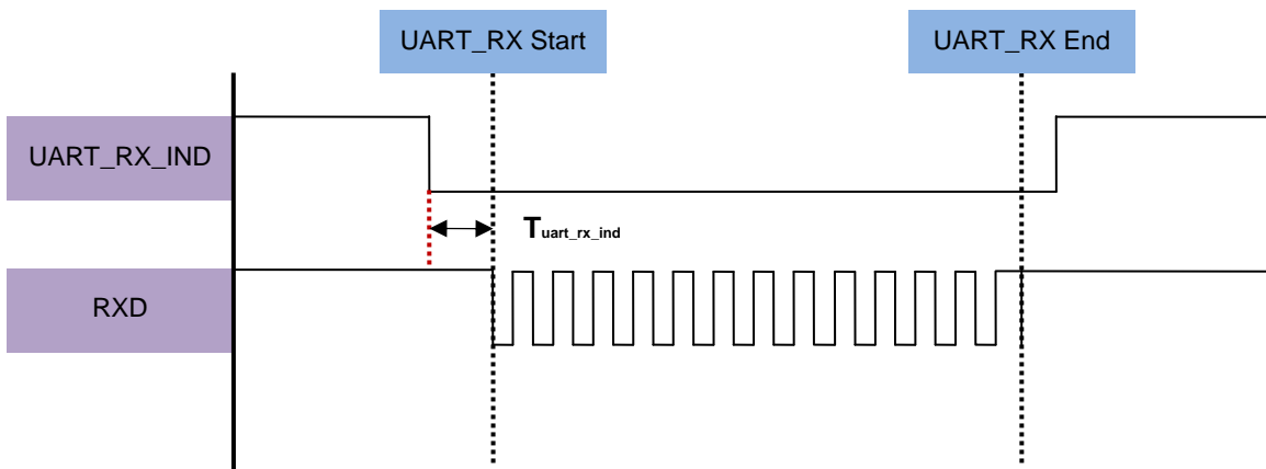
Fig 2.4.1 Host MCU indicate BLEDK3 UART data diagram
